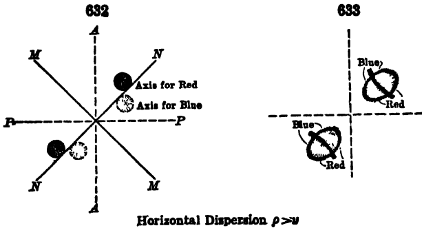
Horizontal Dispersion \rho > \nu
